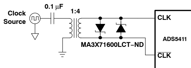
Figure 27. Differential Clock
